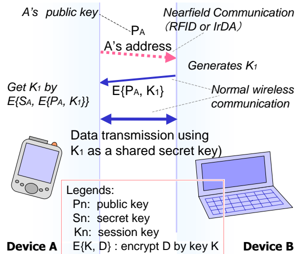
Figure 9: Protocol for establishing secure connection.
